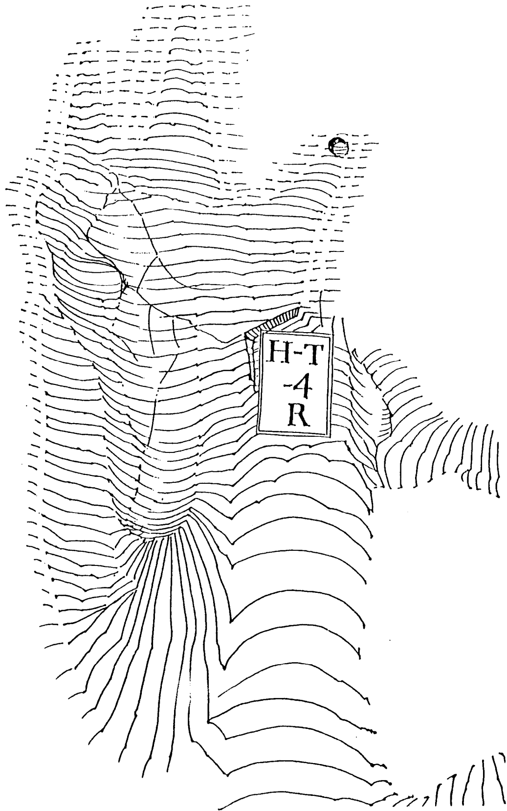
Schematic replication showing primary dinosaur print and secondary print.
